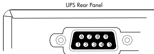
Figure 16 Serial Port
